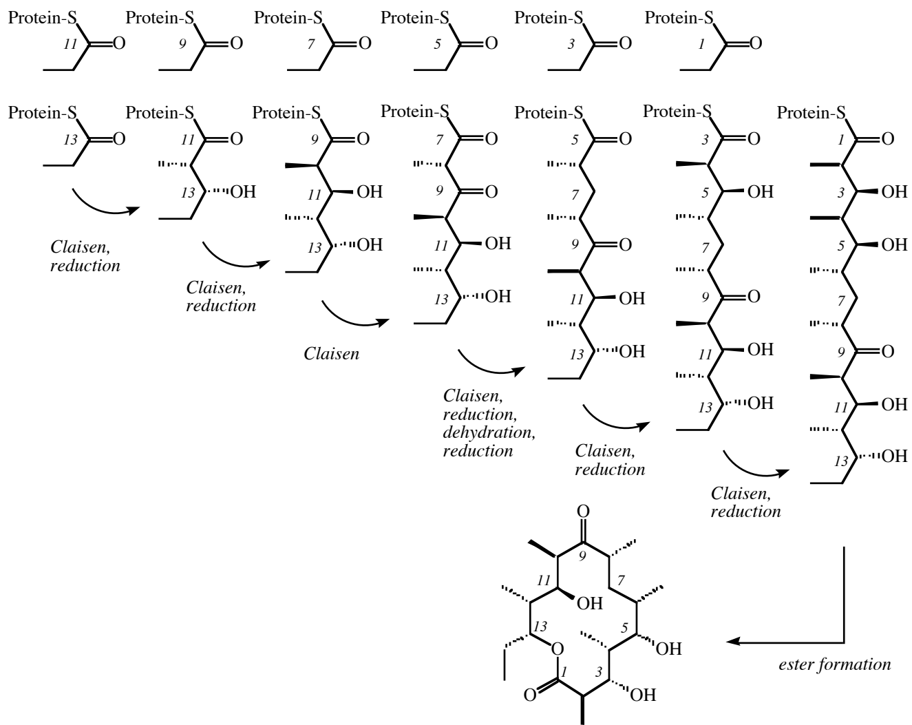
6-Deoxyerythronolide B
